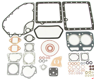
Yanmar 395 Full Set
